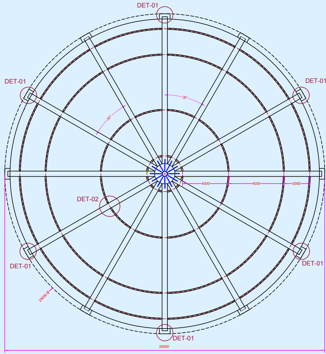
PLAN OF SKYLIGHT AT 6TH FLOOR
