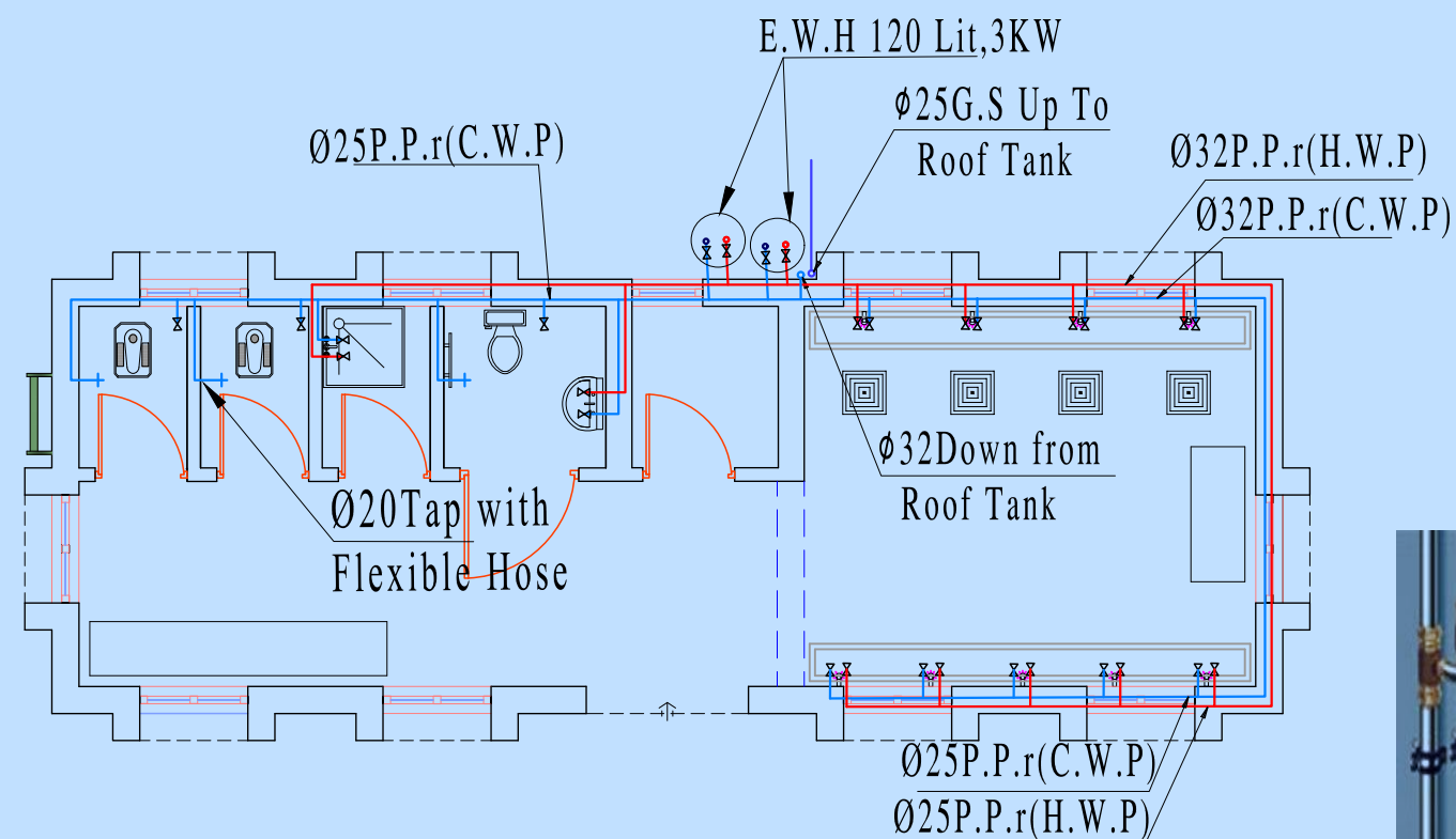
(Hot&Cold Water Supply Plan)
