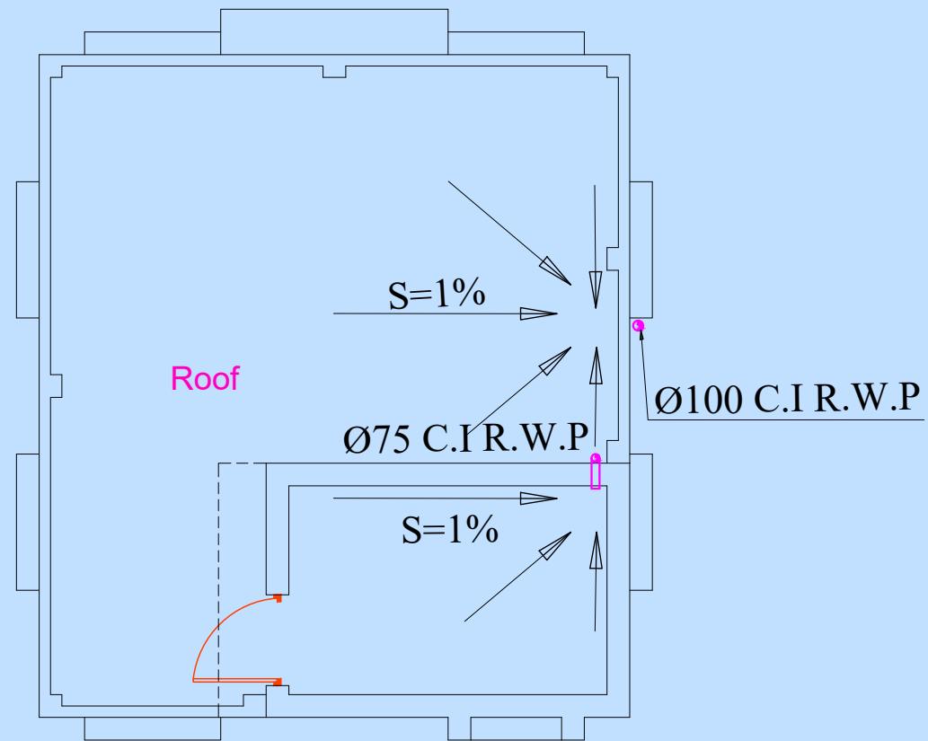
( Rain Water Pipes )
