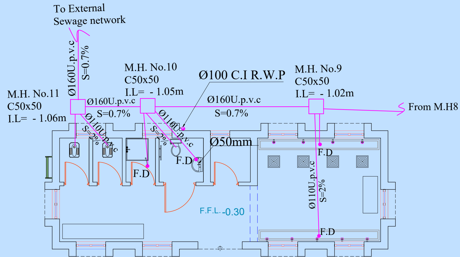
(Drainage Plan )
