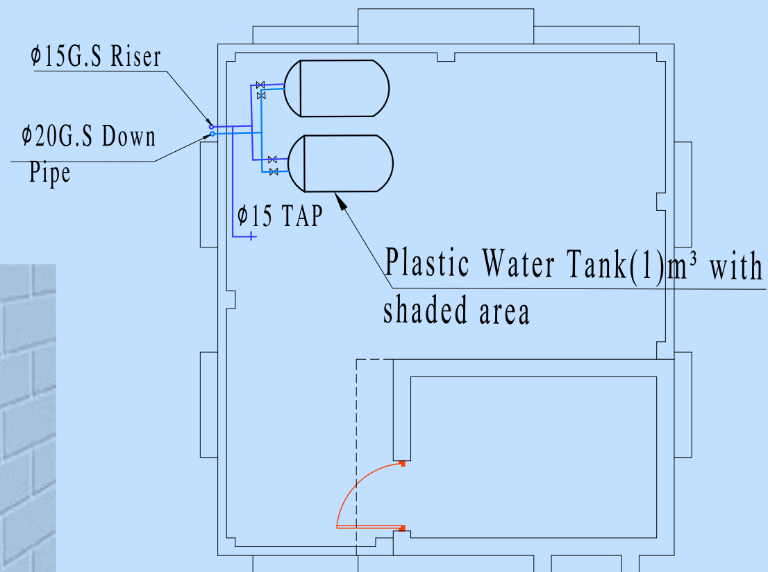
( Water Tanks )
